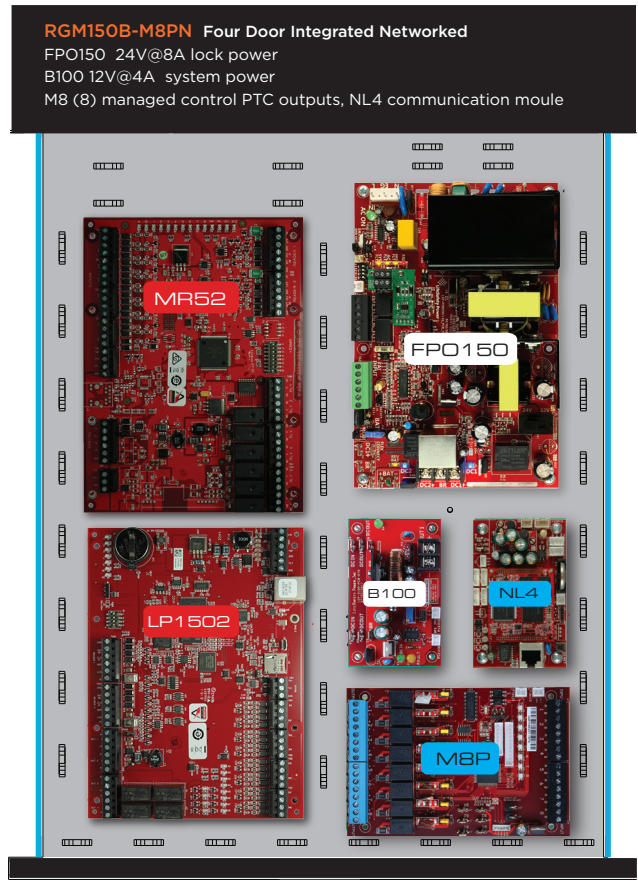
Drawer layout example of 4 door dual voltage managed system
